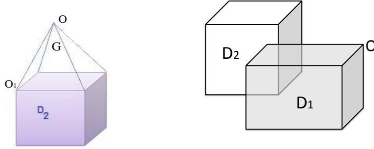
FIGURE 1. Illustration of two different convex polyhedral scatterers. Left: D_2 is a cube and D_1 is the interior of \overline{D_2} \cup G , where G denotes the gap domain between D_1 and D_2 . There are four faces of D_1 around the vertex O , none of them extends to an entire plane in \mathbb{R}^3 \setminus \overline{D_2} . Right: D_1 and D_2 are both cubes. There are three faces of D_1 around the vertex O , only one of them can be extended to an entire plane in \mathbb{R}^3 \setminus \overline{D_2} .
